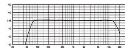
Frequency Response
